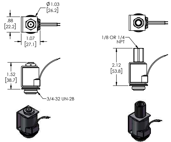
YOKE WITH LEAD WIRES
